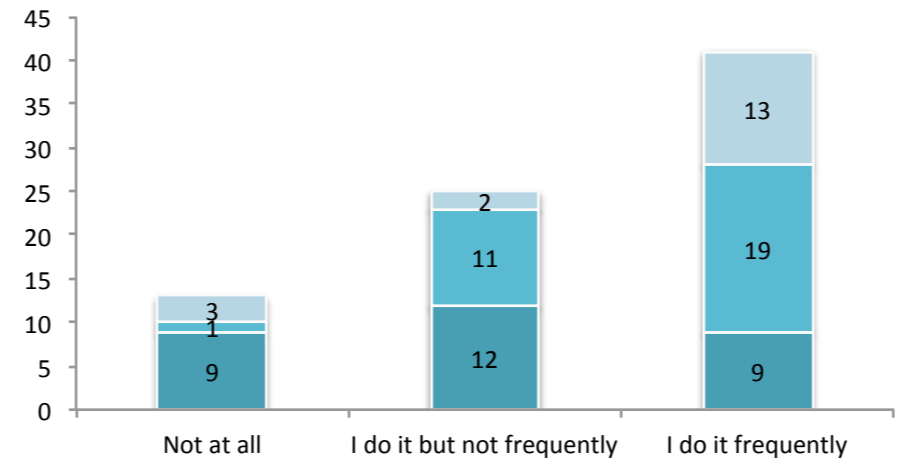
UI Adaptation
